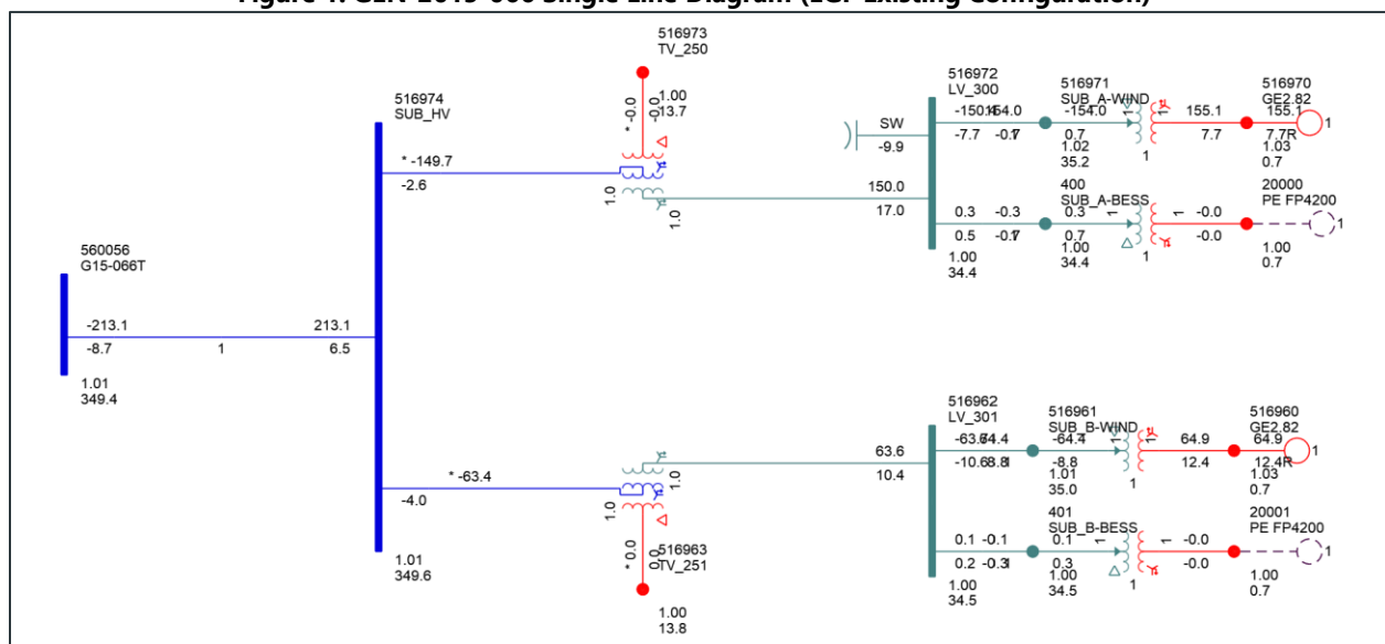
Figure 1: GEN-2015-066 Single Line Diagram (EGF Existing Configuration)
