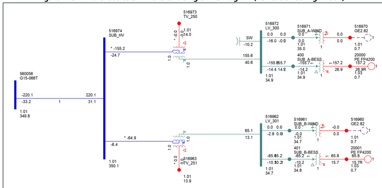
Figure 2: GEN-2015-066 & GEN-2025-SR8 Single Line Diagram (EGF & SGF Configuration)
